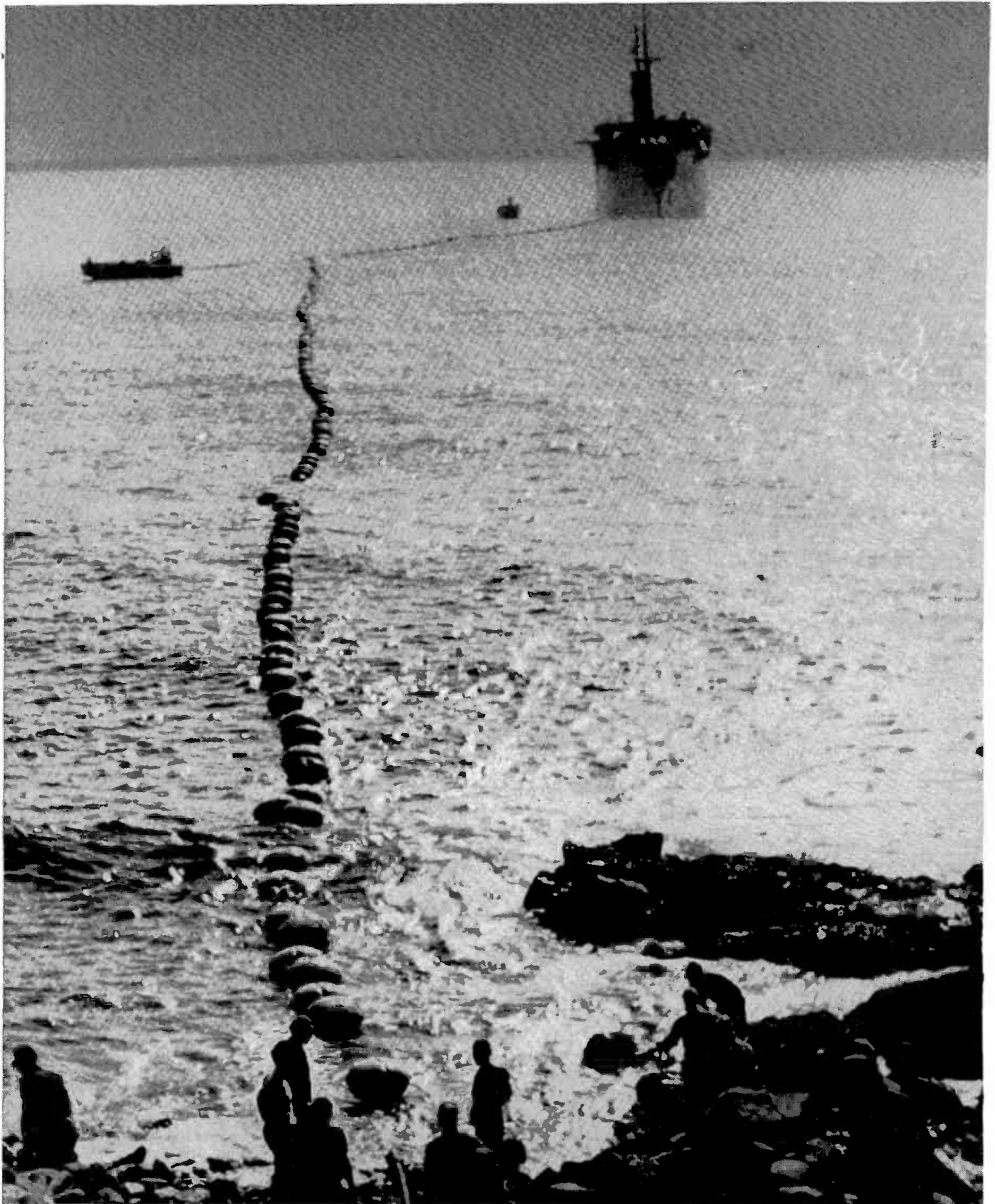
MARKER BUOYS indicate the path of a MILS submarine cable as it is pulled from the cable-laying ship. These are the cables that link MILS shore stations to outlying underwater networks of hydrophones.
